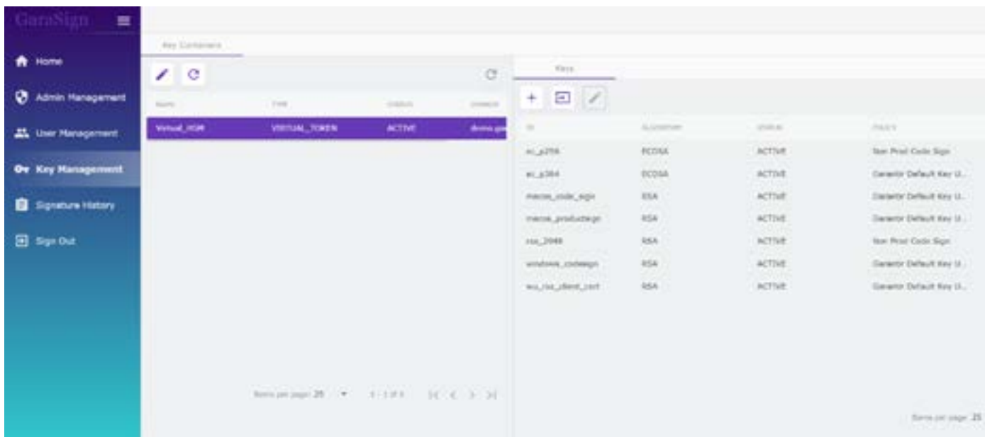
Figure 3 - Menu Expanded
