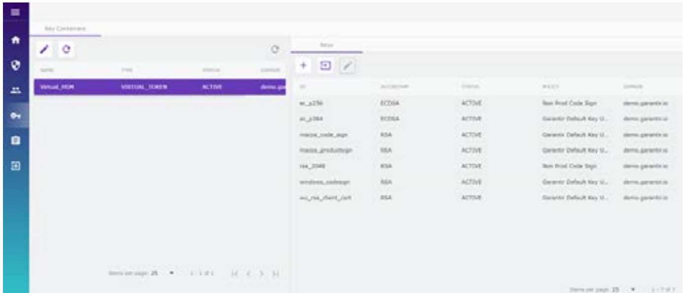
Figure 2 - Menu Collapsed
